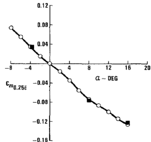
Arrow wing ( M = 0.85 )
